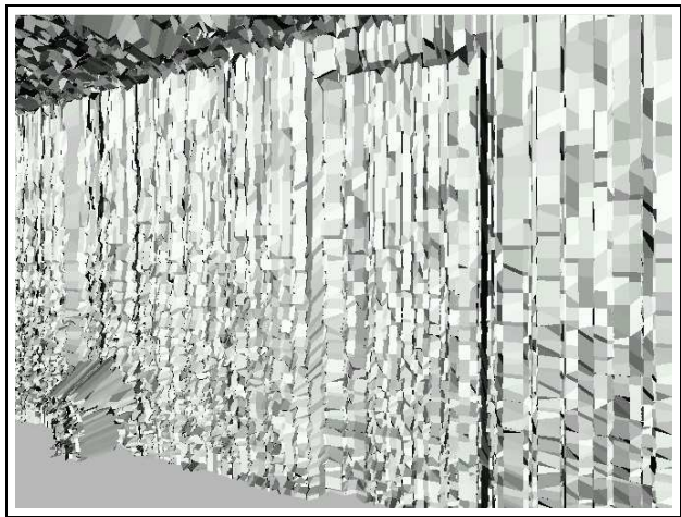
Figure 2: Polygonal model generated from raw data, not using EM. The display without texture shows the level of noise involved, which makes it difficult to separate the door from the nearby wall.
