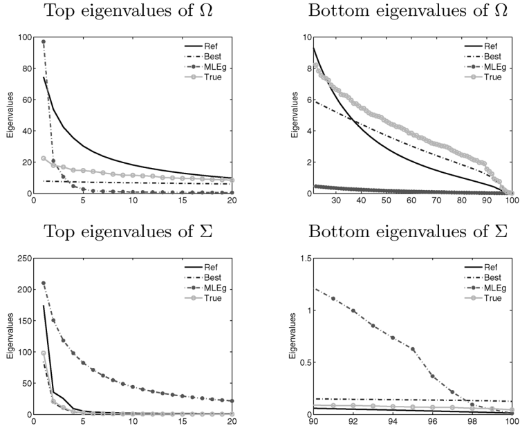
FIG. 1. Scree plots of eigenvalues for \Omega (top row) and \Sigma (bottom row) in the simulation with n = 100 . For each estimator, the lines represent the average of the eigenvalues after 1000 simulations. “Best” refers to the estimator with lowest risk ( IW_{P_G}(1/4c_i, D) ).
